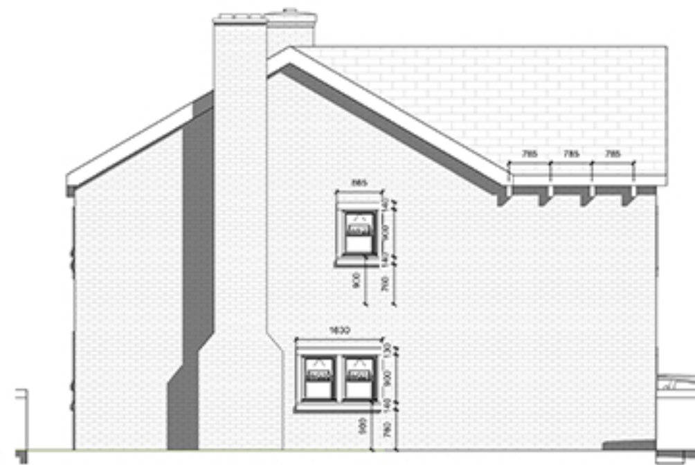
NW side elevation 1:50
