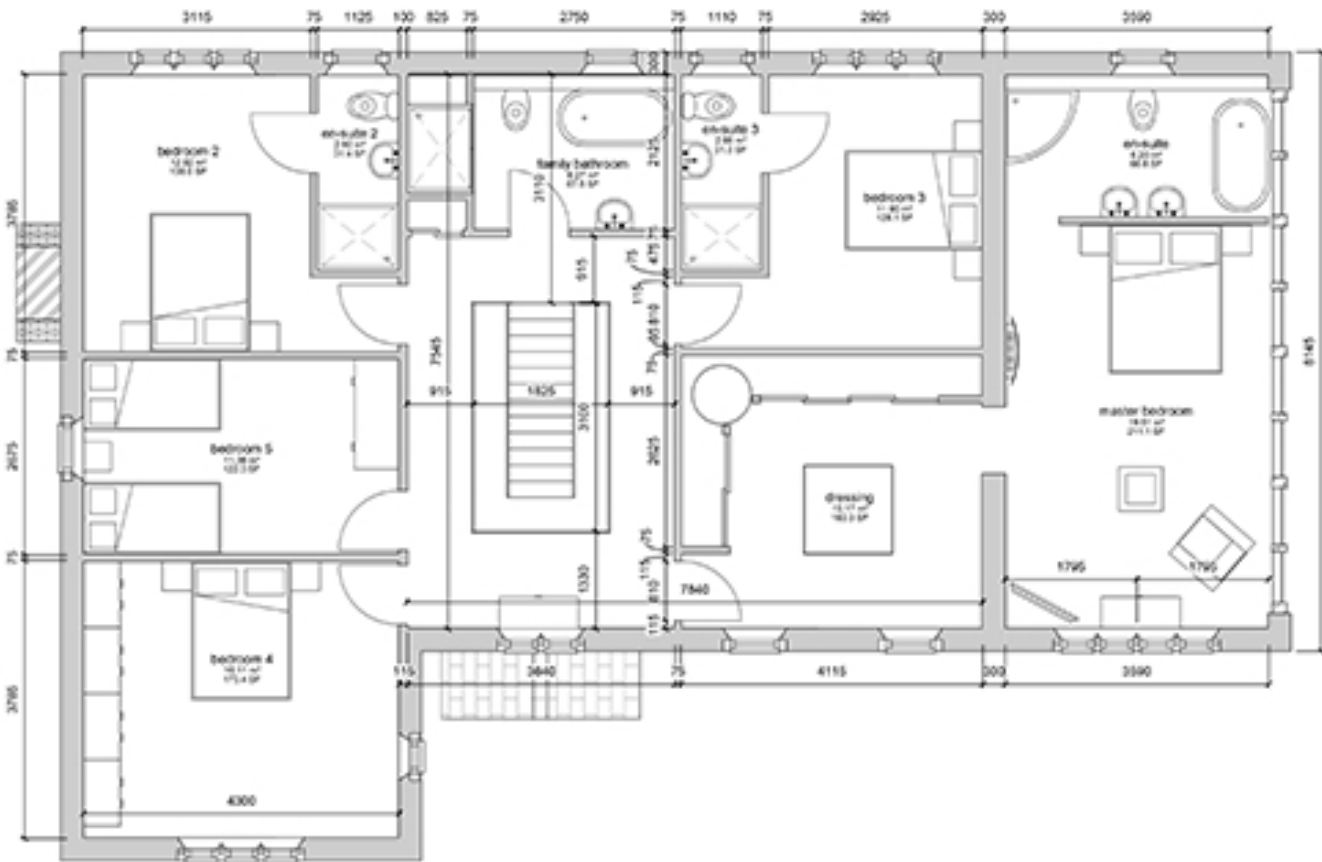
FIRST FLOOR 1:50
